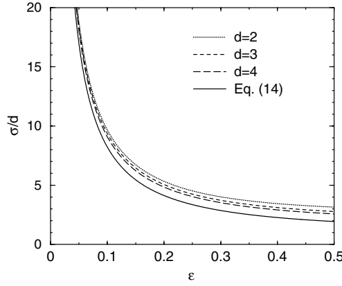
Figure 1. The exact exponent \sigma , obtained from equation (11), versus the dissipation parameter \epsilon . The exponent was scaled by the dimension d . Also shown is the limiting large-dimension expression (14).
